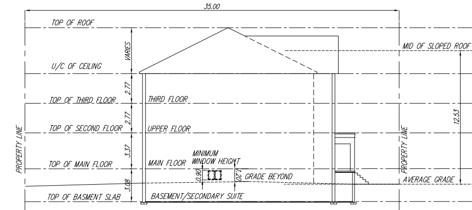
SIDE ELEVATION 7.5M FRONTAGE - 3 STOREY TOWN HOUSE - SPLIT DRAINAGE LOT
