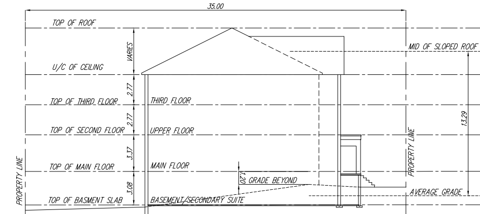
SIDE ELEVATION 7.5M FRONTAGE - 3 STOREY TOWN HOUSE - WALKOUT BASEMENT
