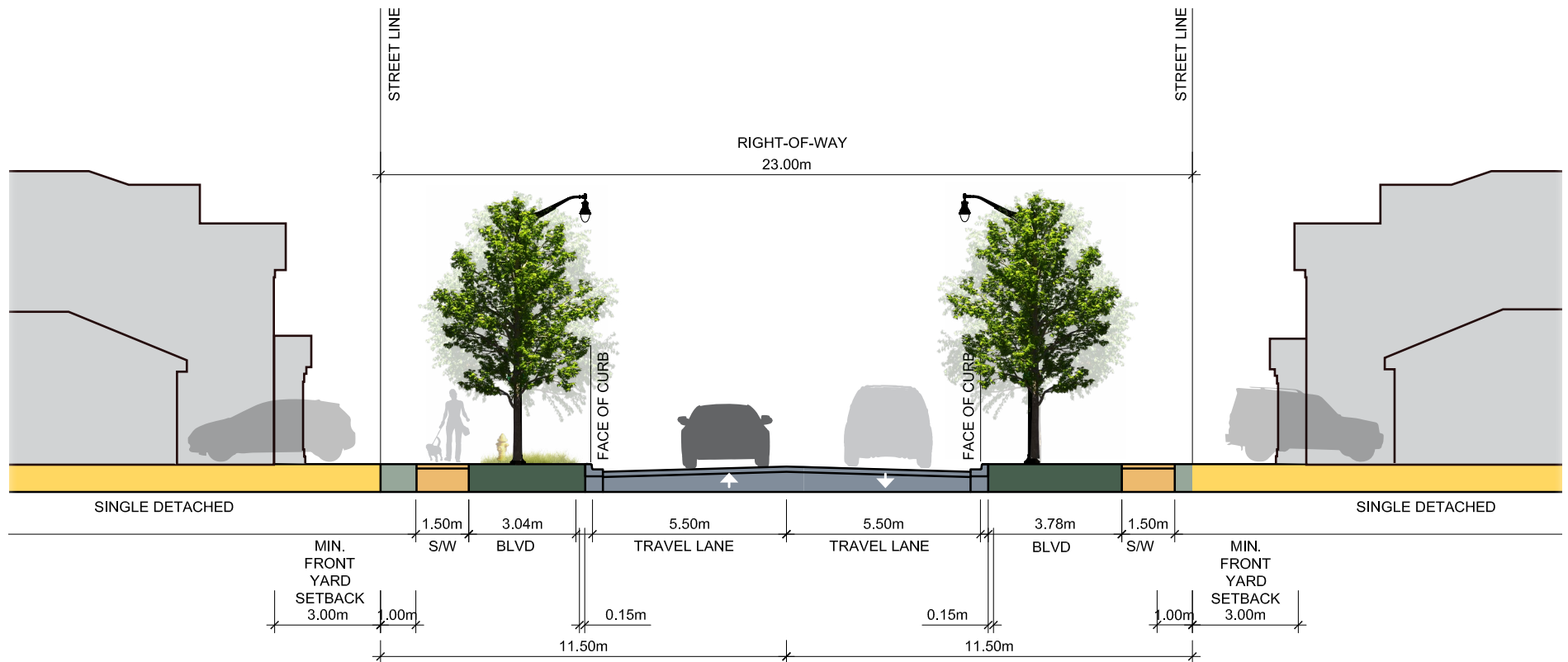
Figure 5: Collector Road 23.0m ROW Cross-section
