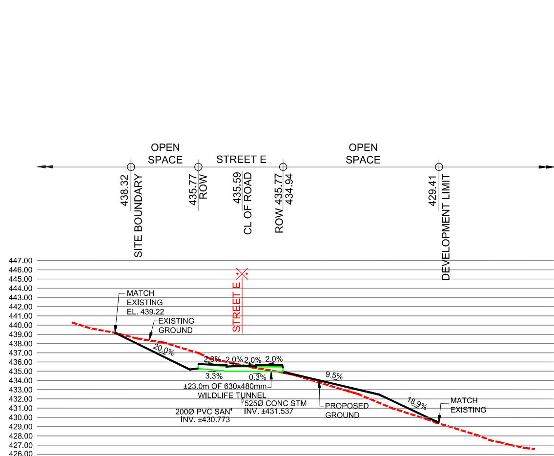
SECTION 3-3 SCALE HOR 1:100 VER 1:40
