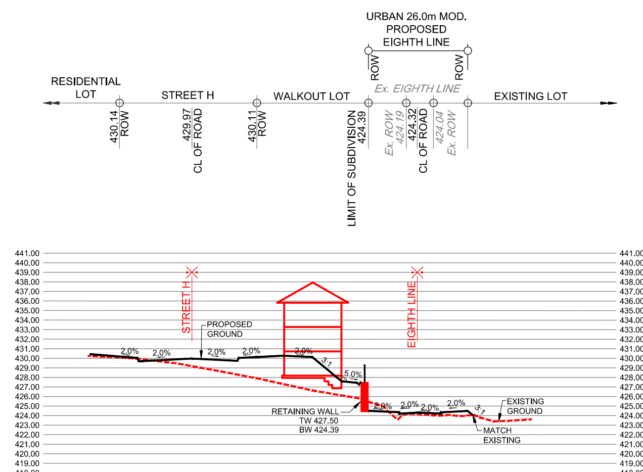
SECTION 5-5 SCALE HOR 1:1000 VER 1:400
