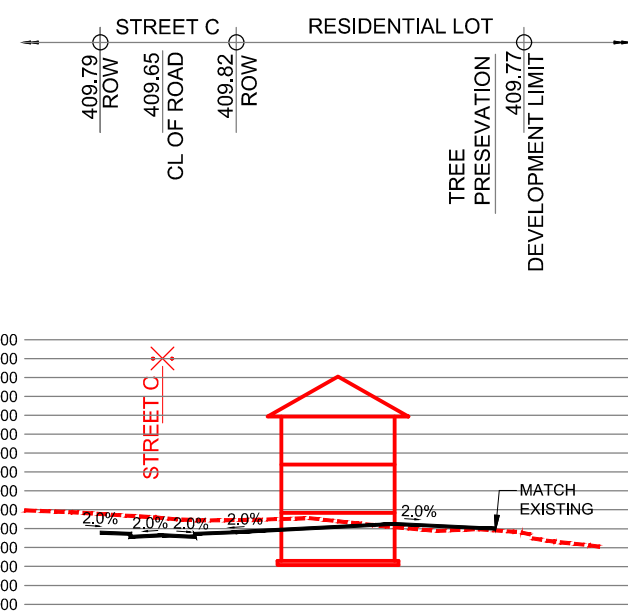
SECTION 1-1 SCALE HOR 1:1000 VER 1:400
