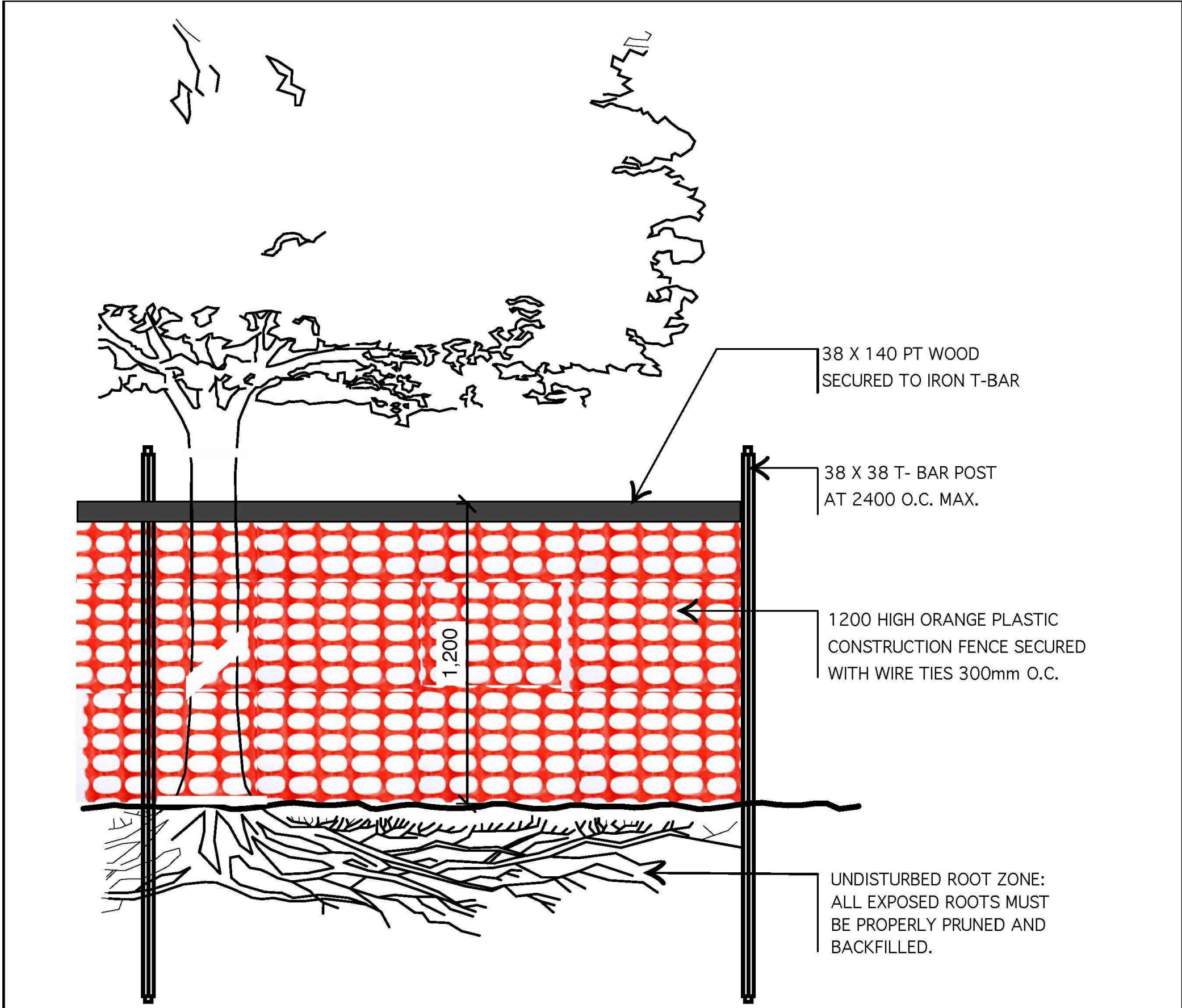
1 TP-4 TREE PROTECTION FENCING DETAIL NTS
