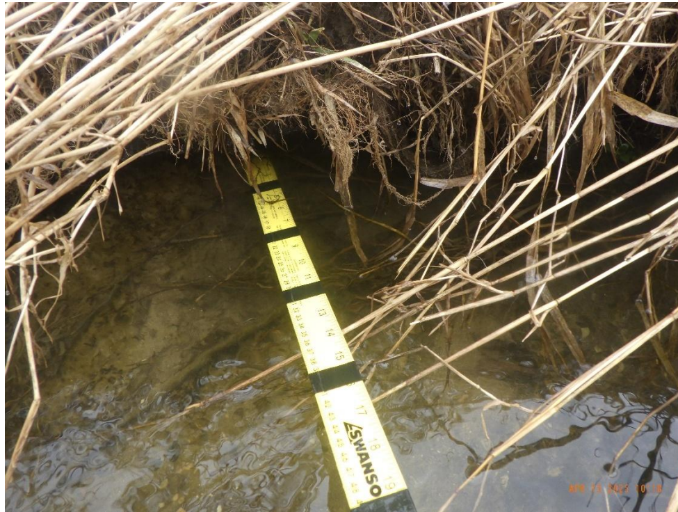
Photograph taken of the edge of channel. Slight undercutting of 0.23m. Meterstick for scale.
