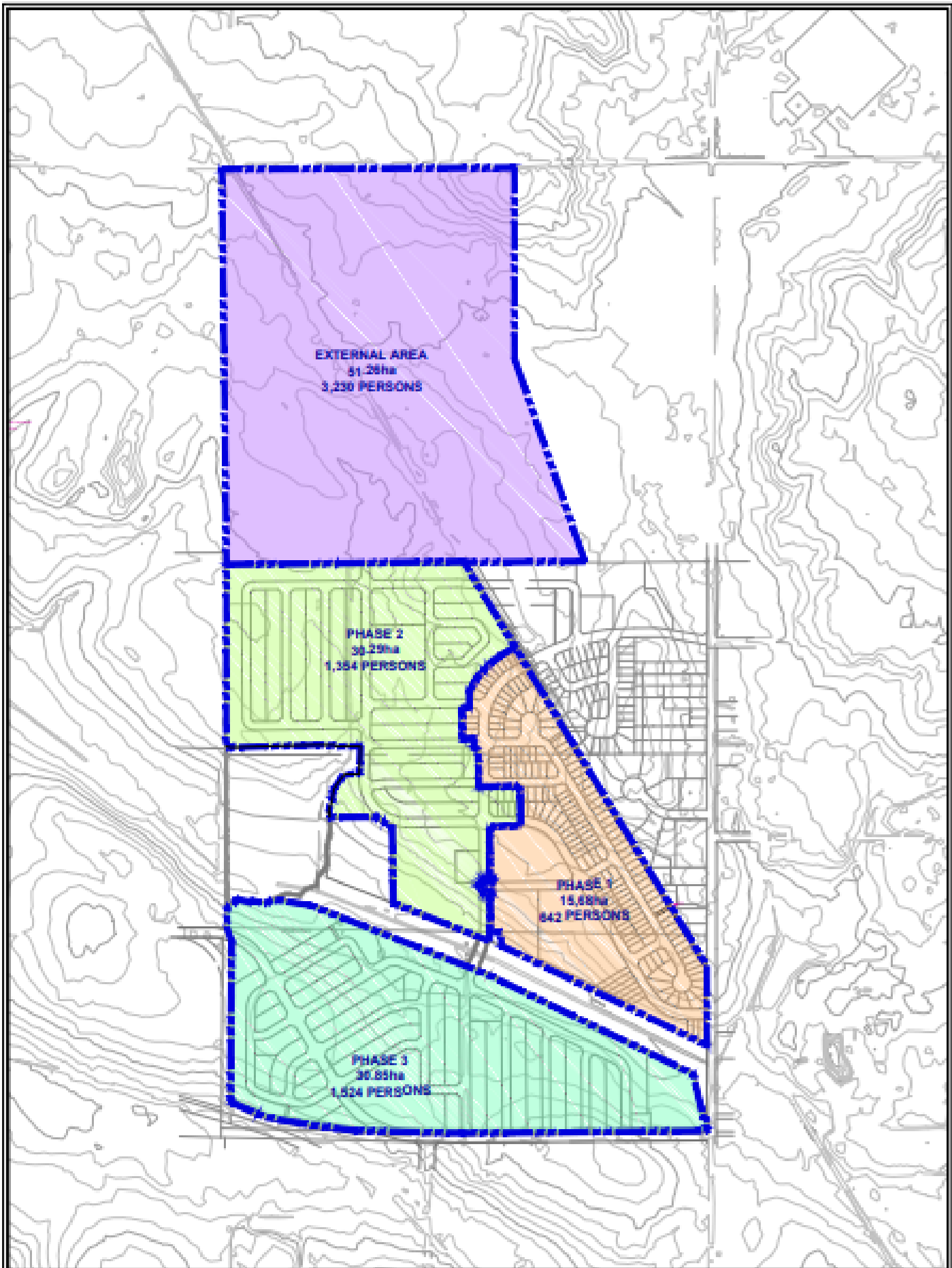
Figure 10a STOREYBROOK SUBDIVISION PROPOSED SANITARY DRAINAGE BOUNDARIES
