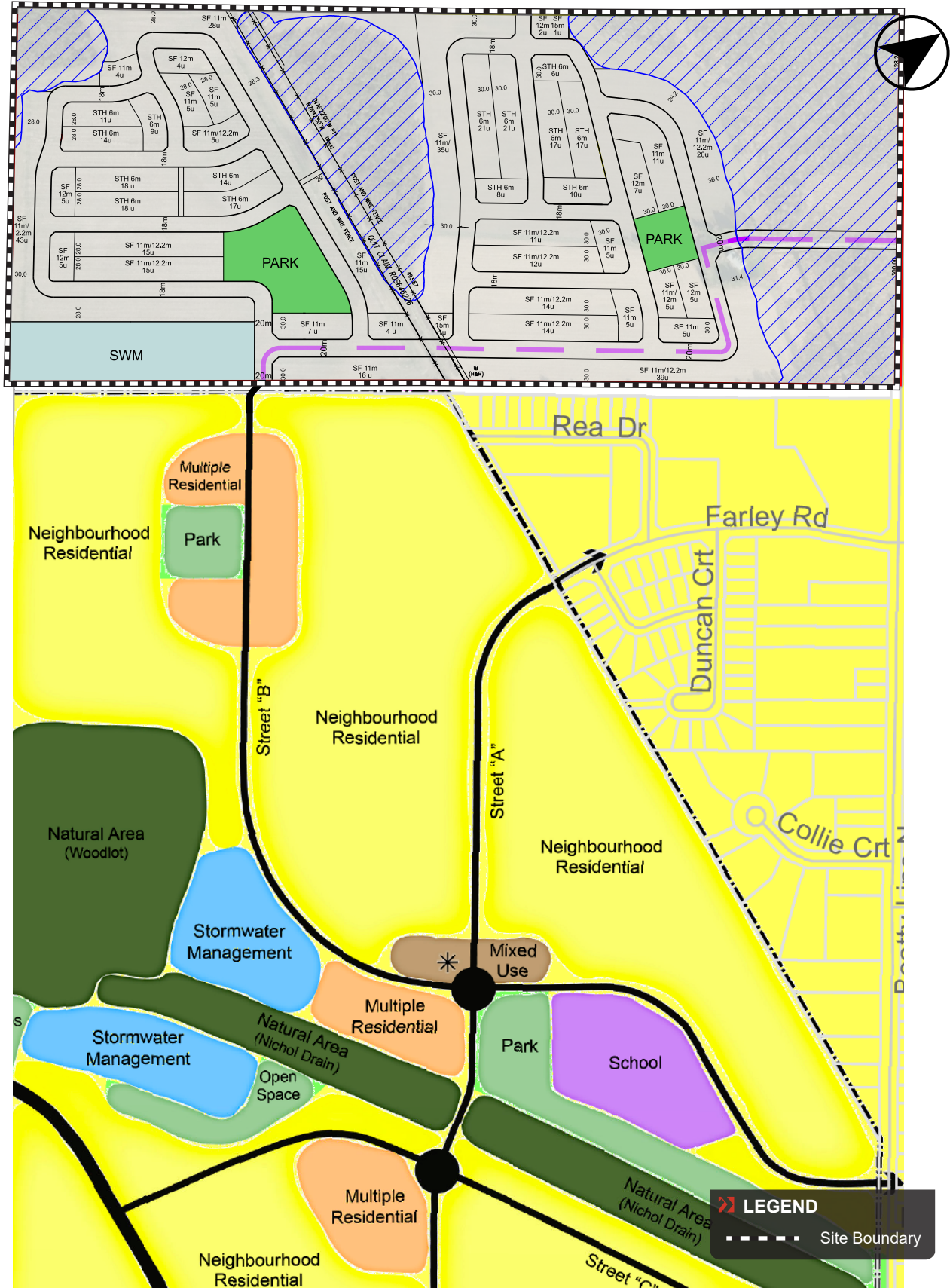
FIGURE 2 SITE PLAN
